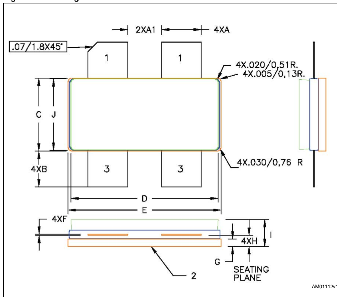
Figure 11. Package dimensions
