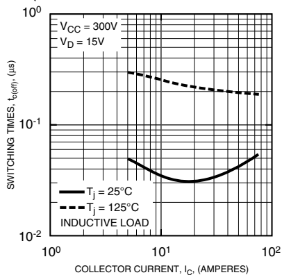
SWITCHING TIME VS. COLLECTOR CURRENT (TYPICAL - LOWER ARM OF CONVERTER PART)
