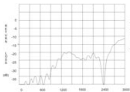
RETURN LOSS (TYPICAL)
