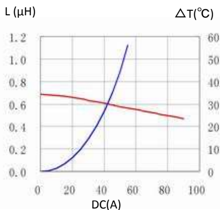
2. 177CDMCCDS-R68MC
