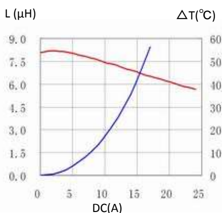
8. 177CDMCCDS-8R2MC
