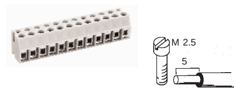
Type 8142 plug-in 90° to wire entry
