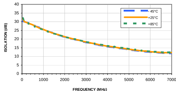
ISOLATION vs. FREQUENCY & TEMPERATURE
