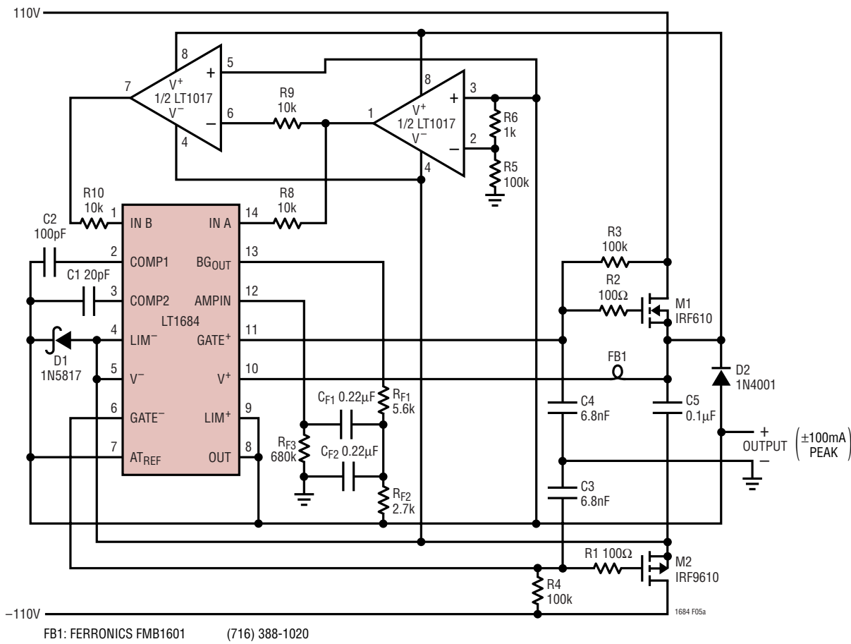
Ringer Output
