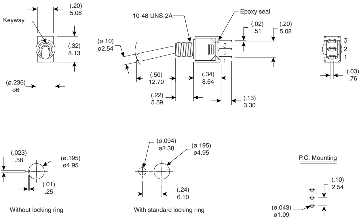
Panel Mounting
