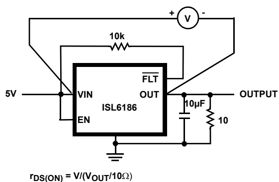
FIGURE 25A. r_{DS(ON)}
