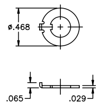
SEALING WASHER U360 1/4-40 For keyway bushing
