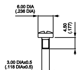
CONNECTING SCREW U03
