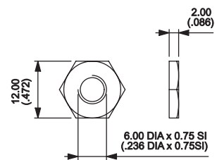
HEX NUT Brass Chrome plated U1916
