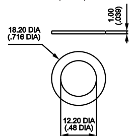
SEALING WASHER Nylon 12mm (.472") U21
