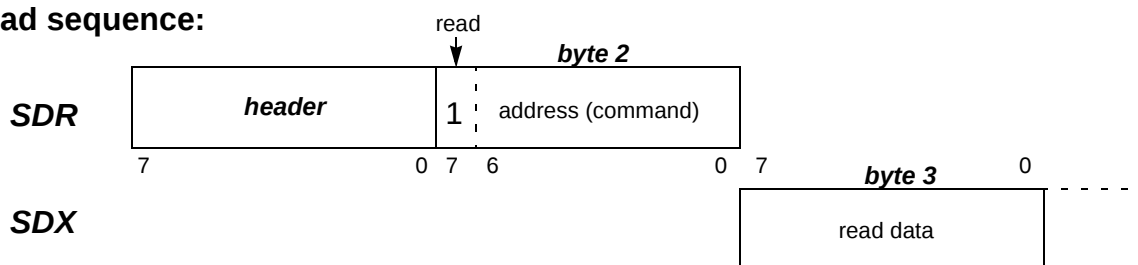
Figure 16 Serial Command Structure
