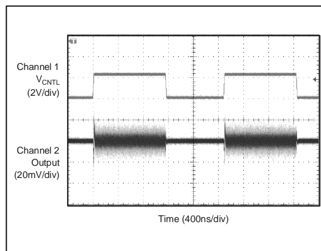
Figure 37. Response to Step Change of V_{\text{CTL}}
