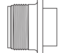
2 Box Mount No Accessory Threads (MS3102)
