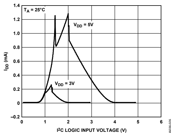
Figure 17 I_{DD} vs. I^2\text{C} Logic Input Voltage (SDA, SCL)
