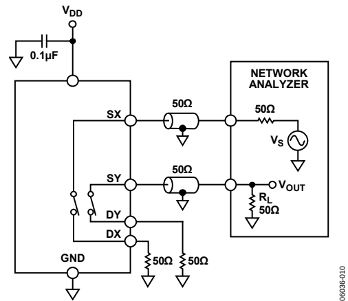
Figure 23. Channel-to-Channel Crosstalk
