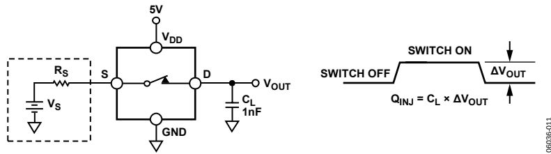
Figure 26. Charge Injection
