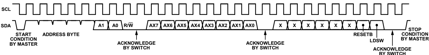
Figure 27. Write Operation
