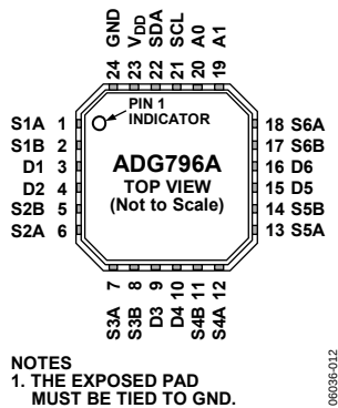
Figure 3. Pin Configuration
