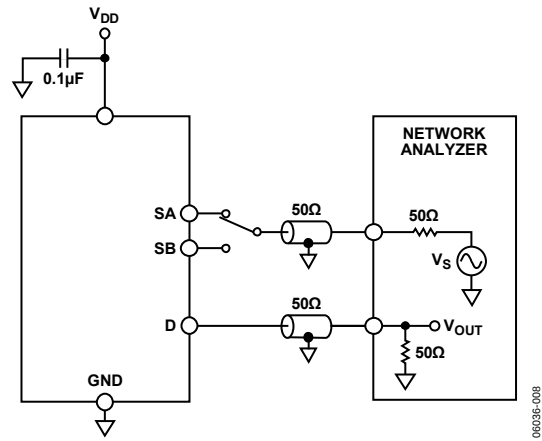
Figure 21. Bandwidth
