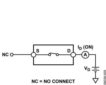
Figure 19. Off Leakage
