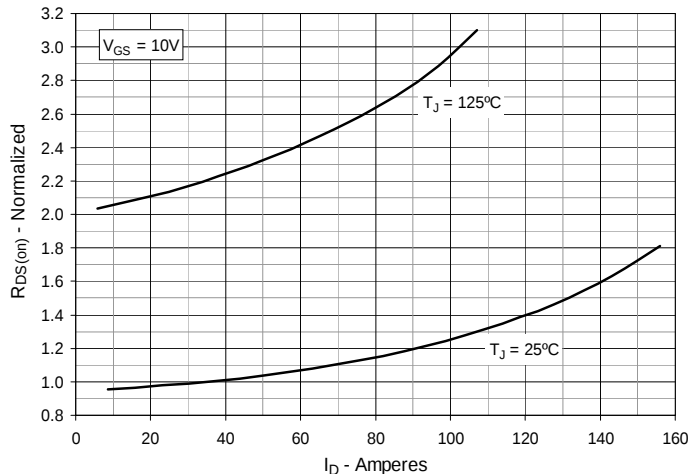
Fig. 5. R_{DS(on)} Normalized to I_D = 39\text{A} Value vs. Drain Current
