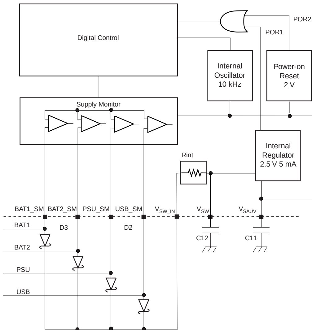
Figure 4. Start-up Overview
