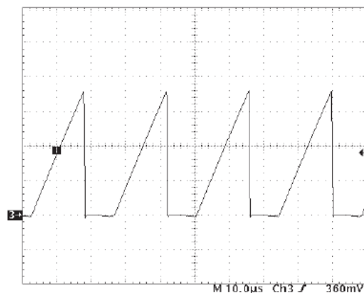
Fig. 7 Transistor Current (200mA/div)
