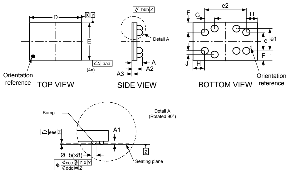
Figure 28. WLCSP8 with BSC - Outline
