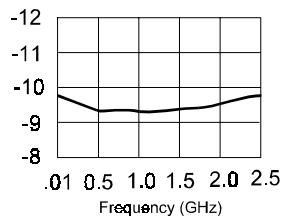
Input Power Flatness (dBm)
