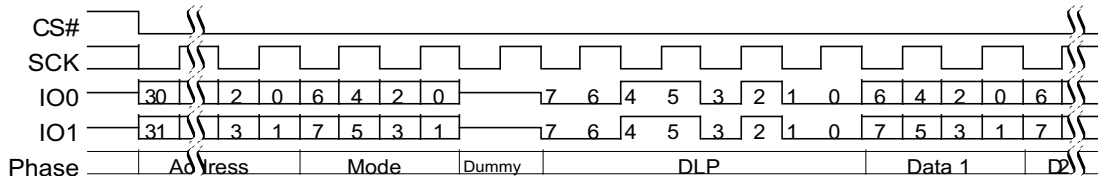
Figure 92. Continuous DDR Dual I/O Read Subsequent Access (4-Byte Address, EHPLC= 01b)
