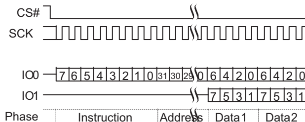
Figure 75. Dual Output Read Command Sequence (4-Byte Address, 3Ch or 3Bh [ExtAdd=1, LC=11b])
