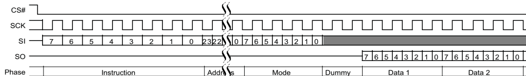
Figure 87. Continuous DDR Fast Read Subsequent Access (3-Byte Address [ExtAdd=0, EHPLC=11b])
