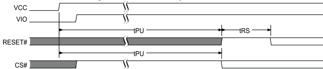
Figure 28. POR followed by Hardware Reset
