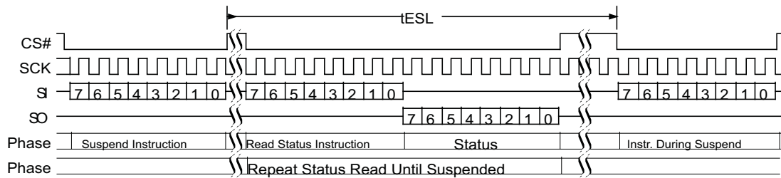
Figure 104. Erase Suspend (ERSP 75h) Command Sequence
