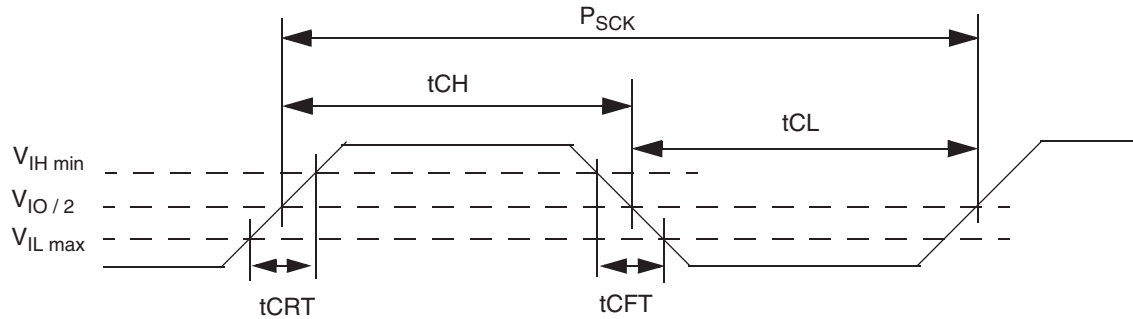
Figure 30. Clock Timing
