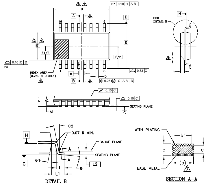
Figure 40. SOIC 16-Lead, 300-mil Body Width (SO3016)
