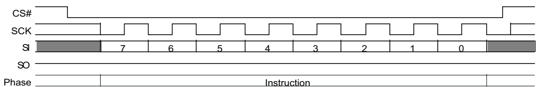
Figure 105. Erase Resume (ERRS 7Ah) Command Sequence
