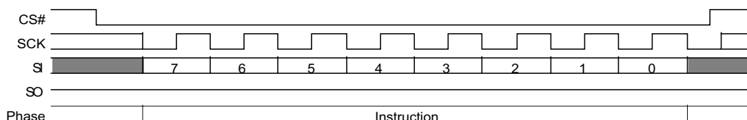
Figure 120. Software Reset (RESET F0h) Command Sequence
