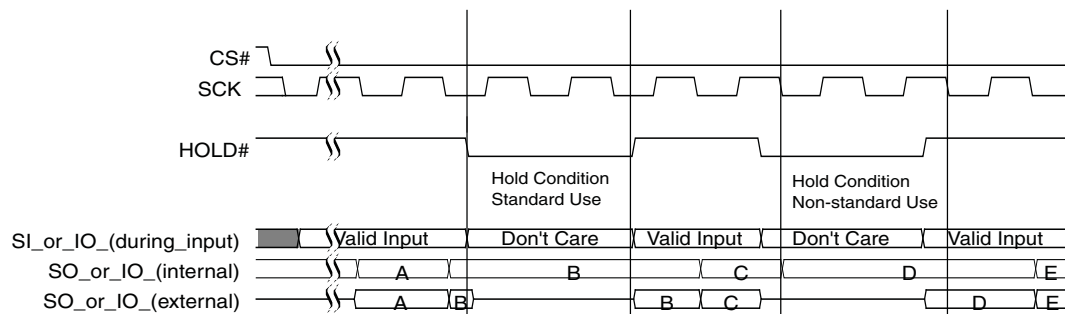
Figure 1. HOLD Mode Operation
