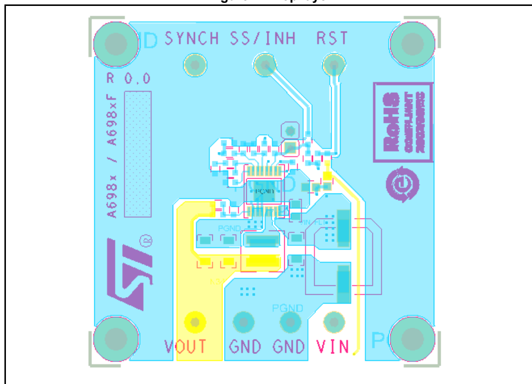
Figure 41. Top layer
