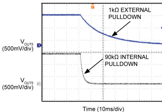
Figure 13. Output Pull-Down Resistance
