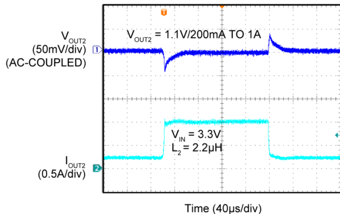
Buck 2 Load Transient – 200mA to 1A
