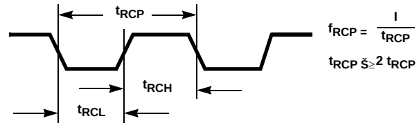
FIGURE 55. REFCLK
