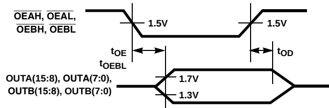
FIGURE 53. OUTPUT ENABLE/DISABLE
