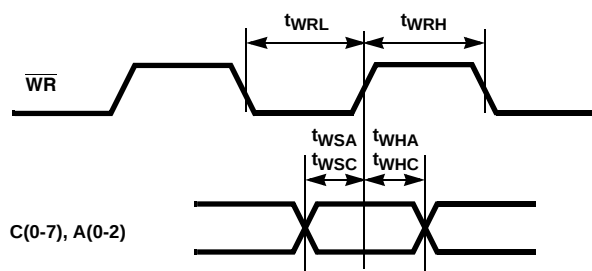
FIGURE 49. TIMING RELATIVE TO \overline{WR}
