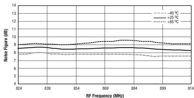
Figure 6. Noise Figure vs Frequency and Temperature
