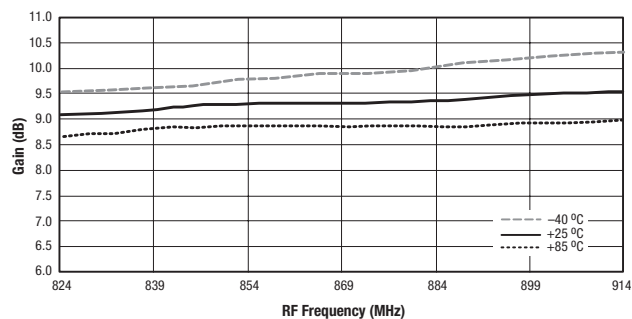
Figure 4. Gain vs Frequency and Temperature
