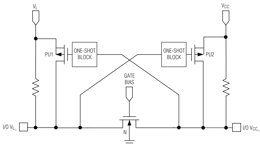
Figure 2b. Functional Diagram, MAX3373E/MAX3378E (1 I/O line)
