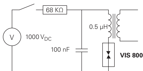
VIS 800 Life Test Circuit
