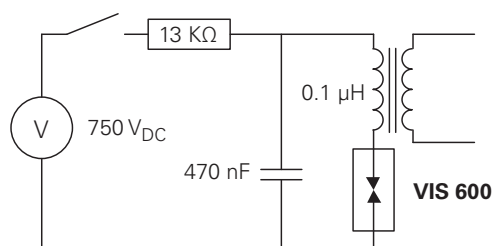
VIS 600 Life Test Circuit
