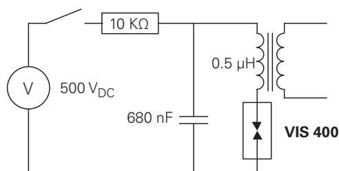
VIS 400 Life Test Circuit
