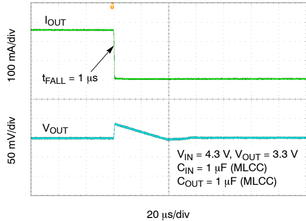
Figure 33. Load Transient Response – 250 mA to 1 mA – V OUT = 3.3 V
