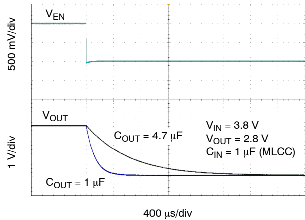
Figure 35. Enable Turn-off
