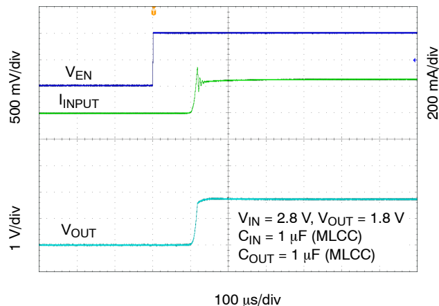
Figure 26. Enable Turn-on Response – C_{OUT} = 1 \mu\text{F} , I_{OUT} = 250 \text{ mA}
