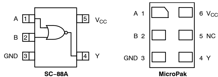
Figure 1. Pinout Diagrams (Top Views)
