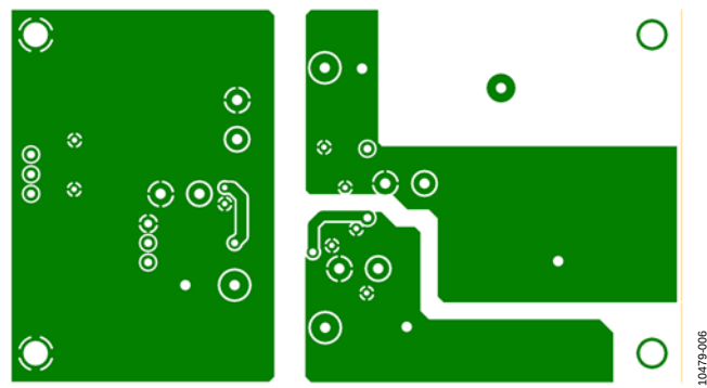
Figure 6. Bottom Layer
