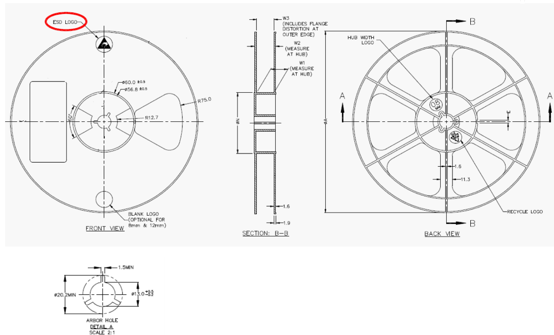
Figure 27. Flip-Chip 8 (1.14x1.44 mm) reel outline
