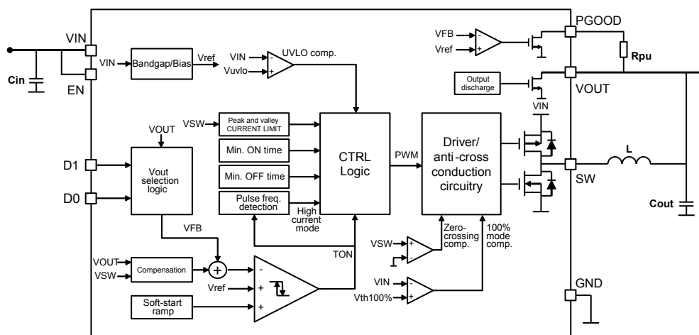
Figure 3. Block diagram
