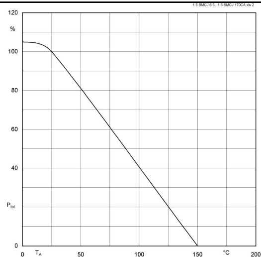
Fig. 2 Rated power dissipation vs. ambient temperature 2)
