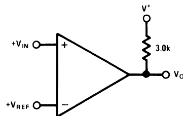
FIGURE 1. Basic Comparator
