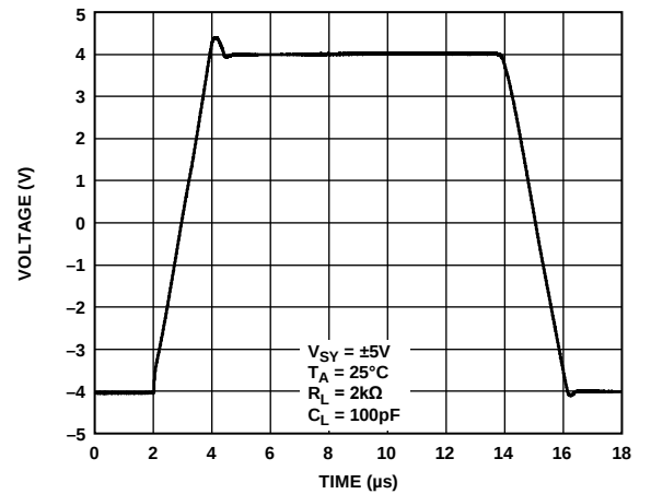
Figure 49. Large Signal Transient Response
