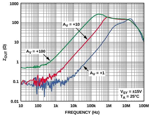
Figure 74. Output Impedance vs. Frequency
