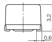
Type FB (4.5×3.2×3.2)
