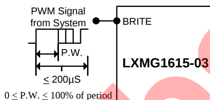
Figure 5A - PWM Brightness Control
