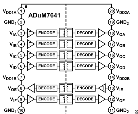
Figure 2. ADuM7641
