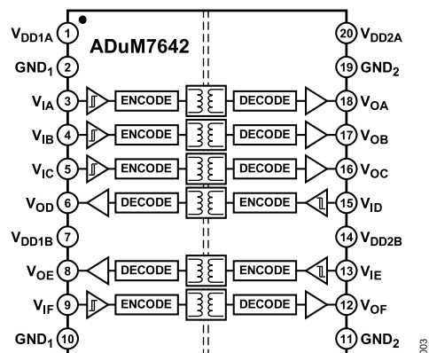
Figure 3. ADuM7642
