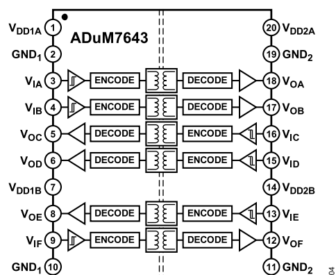
Figure 4. ADuM7643
