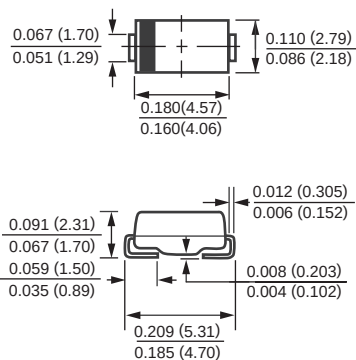
DO-214AC
