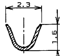
断面 "C"- "C" SECT.
