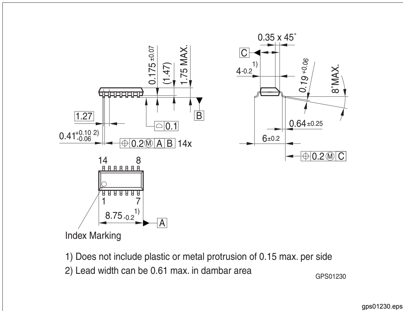
Figure 8 PG-DSO-14
