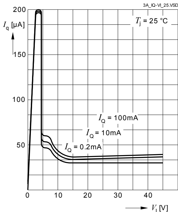
Current Consumption I_q versus Input Voltage V_i at T_j=25\text{°C} (EN=ON)
