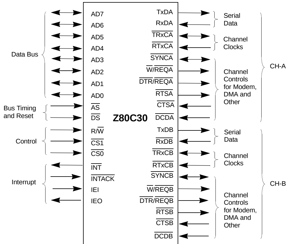
Figure 5.Z80C30 Pin Functions
