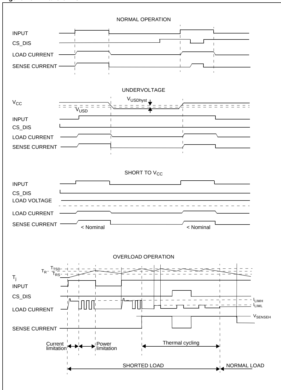
Figure 10. Waveforms
