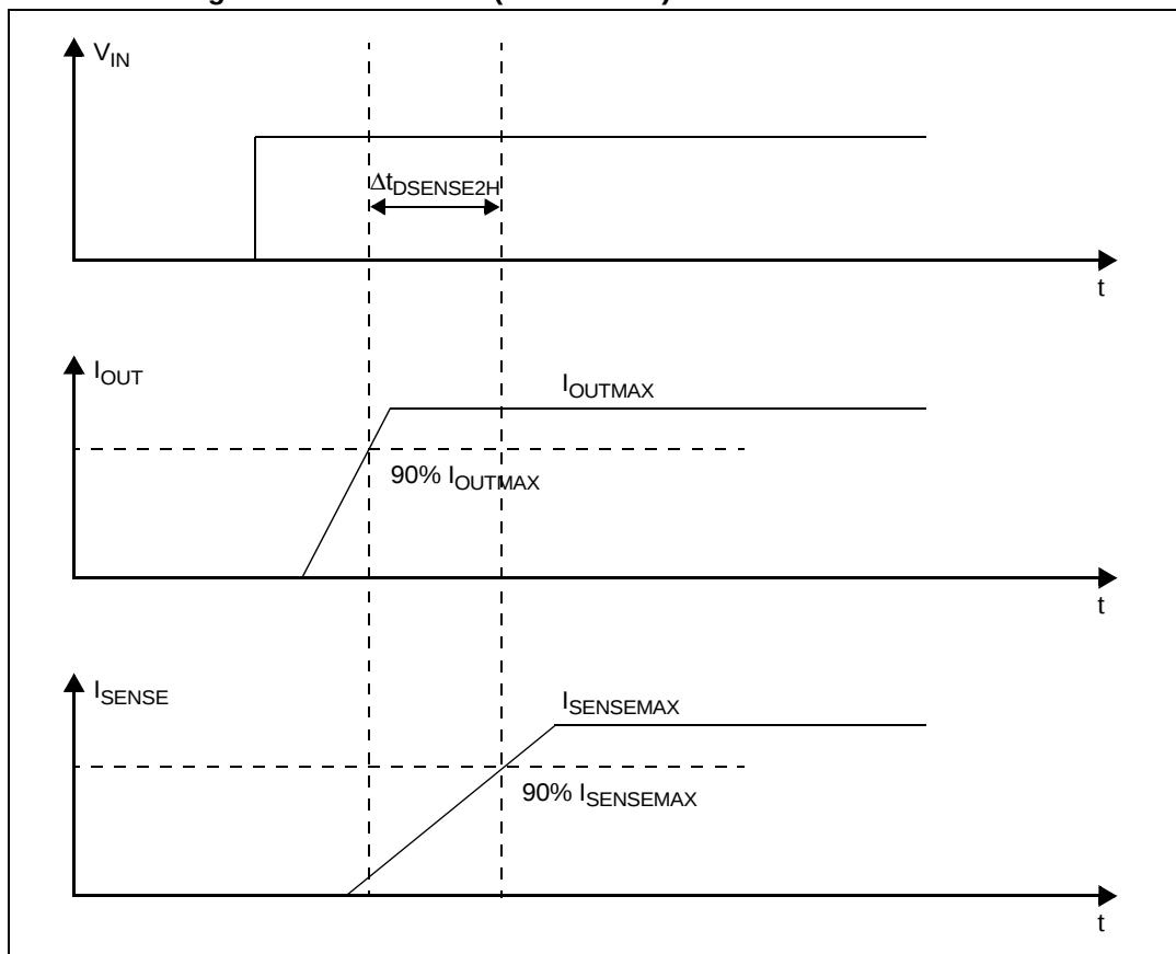
Figure 6. Switching characteristics
