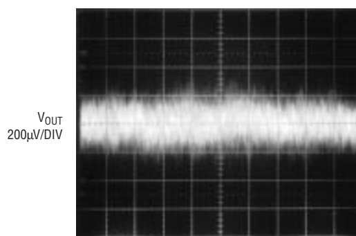
Output Noise (BW = 10Hz to 2.5MHz)
