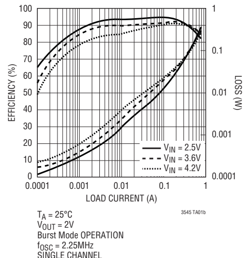
Efficiency and Loss vs Load Current
