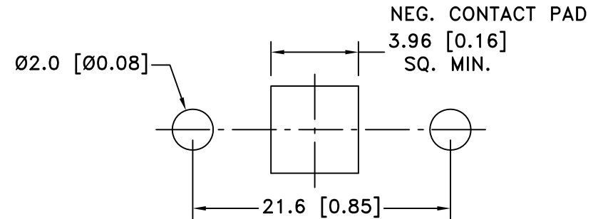
PCB LAYOUT
