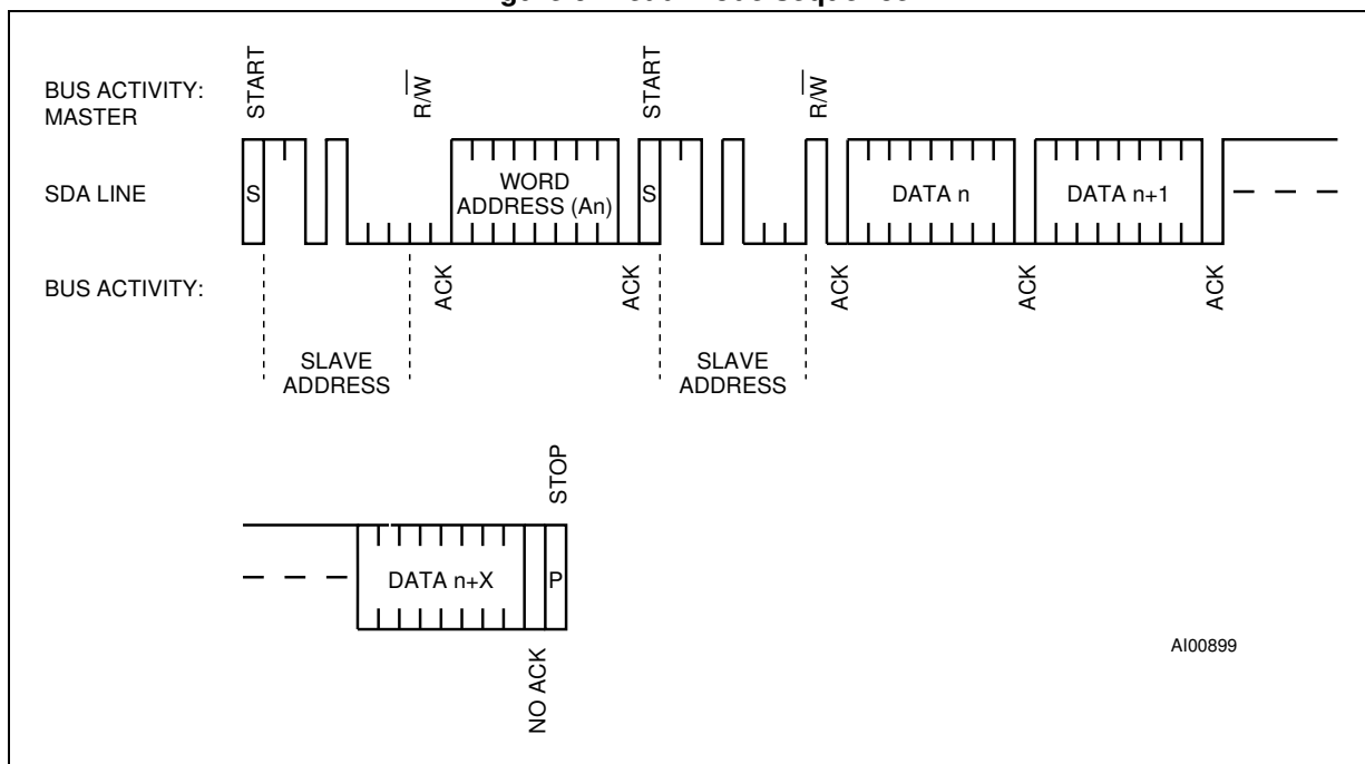
Figure 9. Read mode sequence
