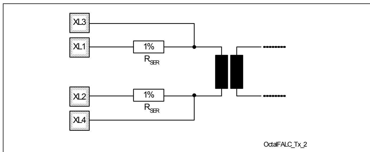
Figure 29 Transmit Impedances
