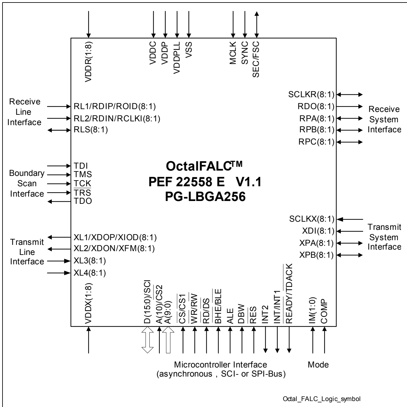
Figure 1 Logic Symbol
