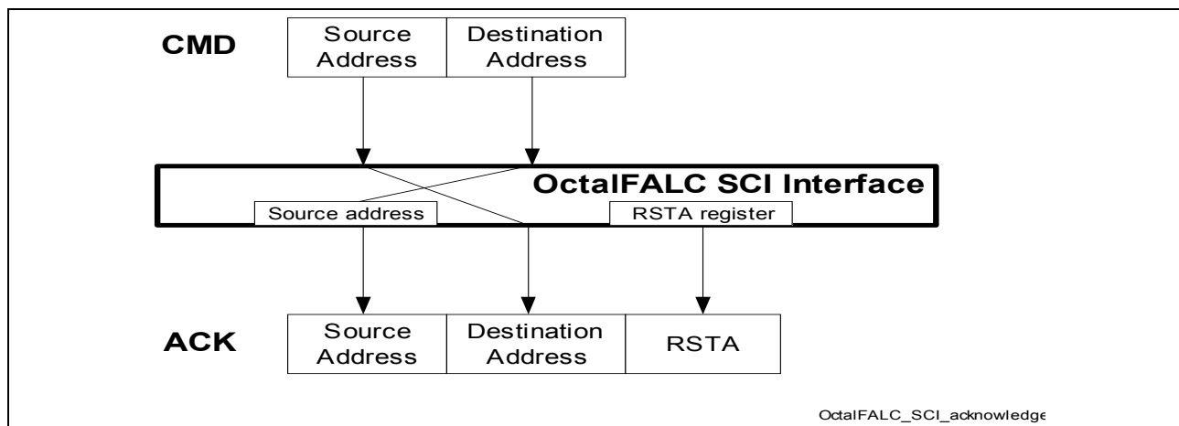
Figure 13 Principle of Building of Addresses and RSTA Bytes in the SCI ACK Message
