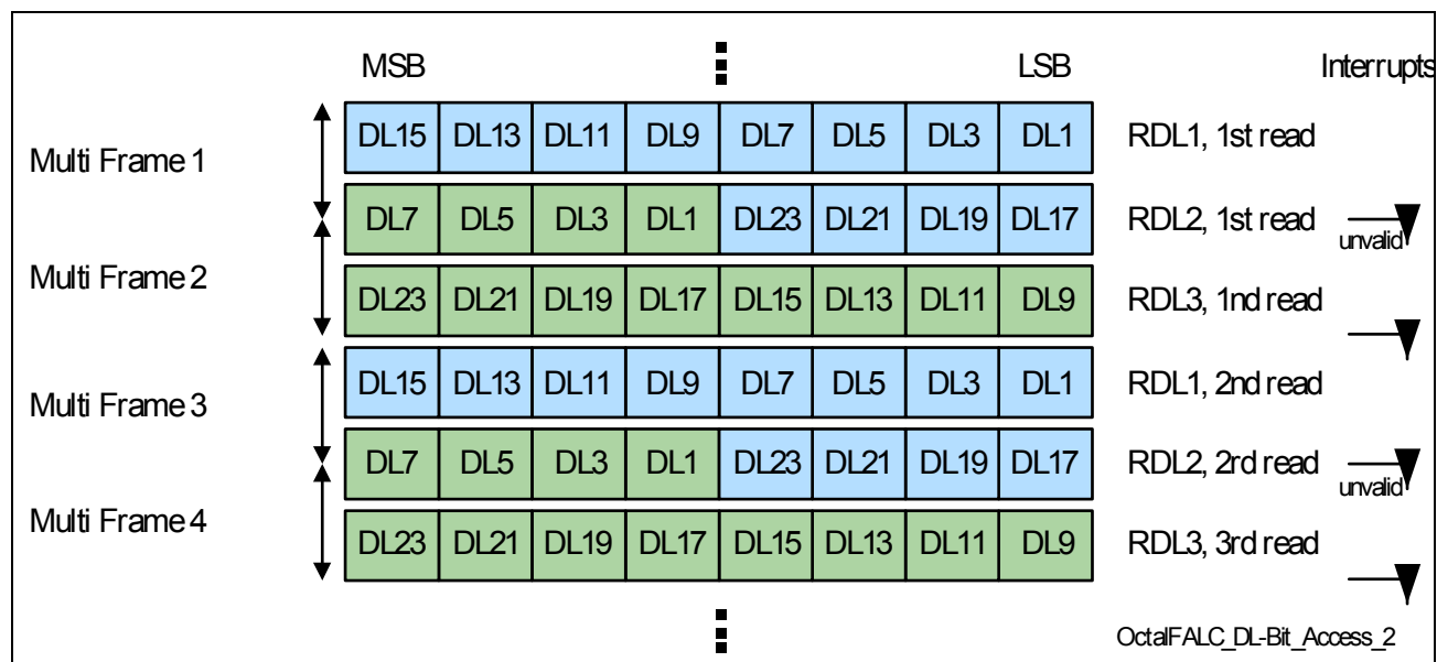
Figure 23 Optional DL-Bit Access in ESF Mode
