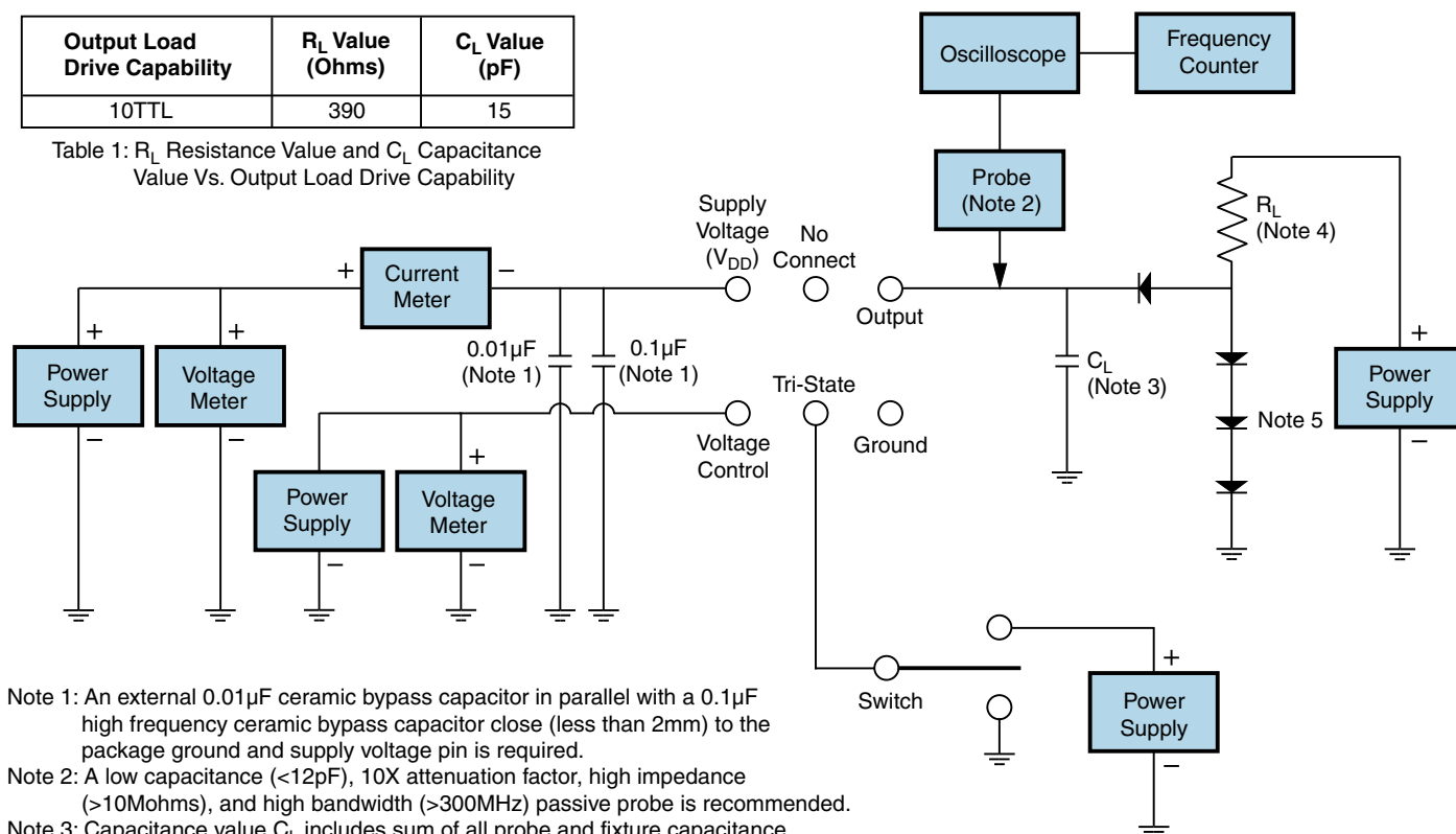
Test Circuit for TTL Output
