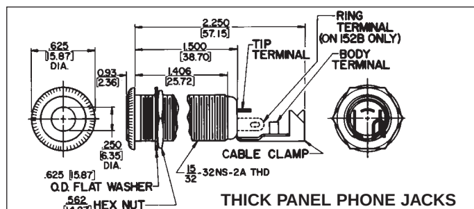
THICK PANEL PHONE JACKS
