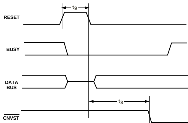
Figure 13. RESET Timing
