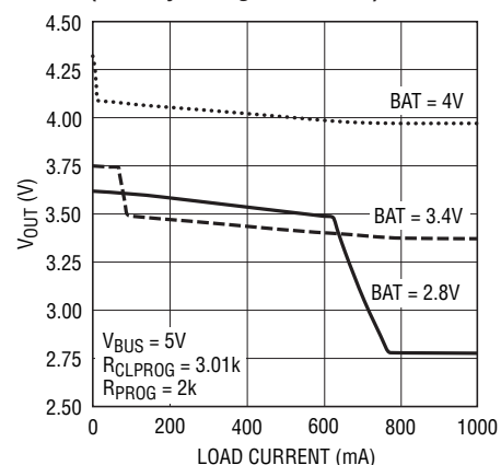
V_{OUT} Voltage vs Load Current (Battery Charger Enabled)
